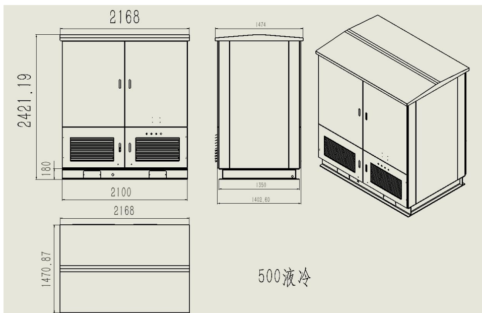
Outdoor Cabinet Size Drawing
