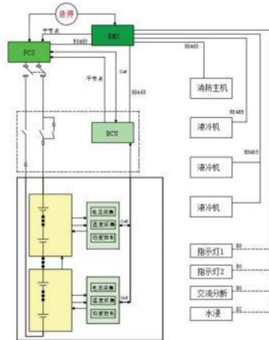
Figure 2-3 Schematic Diagram of BMS Communication Architecture
